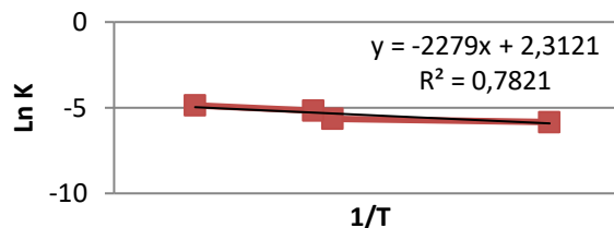
Figure 3. Graph of \ln K with 1/T
