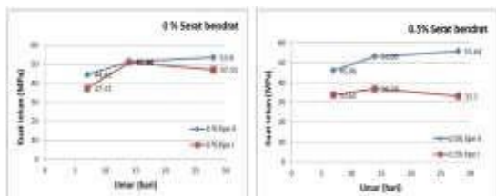
Figure 4. Graph of the Relationship Between Age and Concrete Compressive Strength
